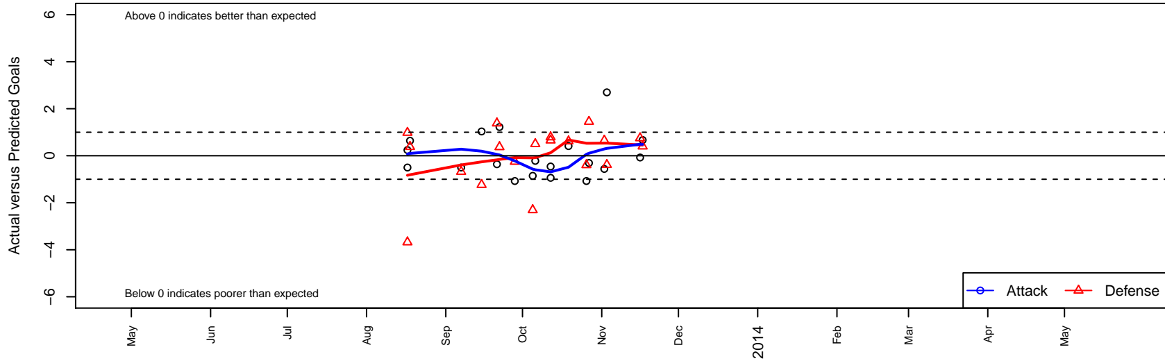
Real So Cal White G00 Dots are actual minus expected GF (blue circles) and GA (red triangles). Blue line is smoothed change in attack strength. Red is smoothed change in defense strength.
